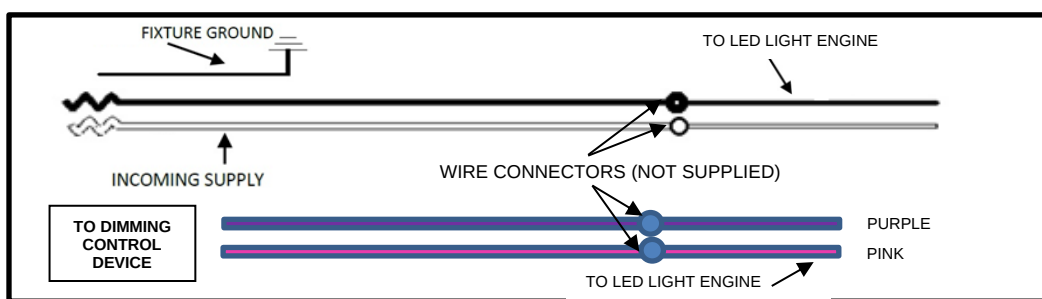
FIG 5: WIRING DIAGRAM
