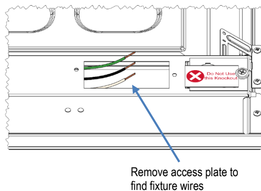
FIG 4: WIRE LOCATION
