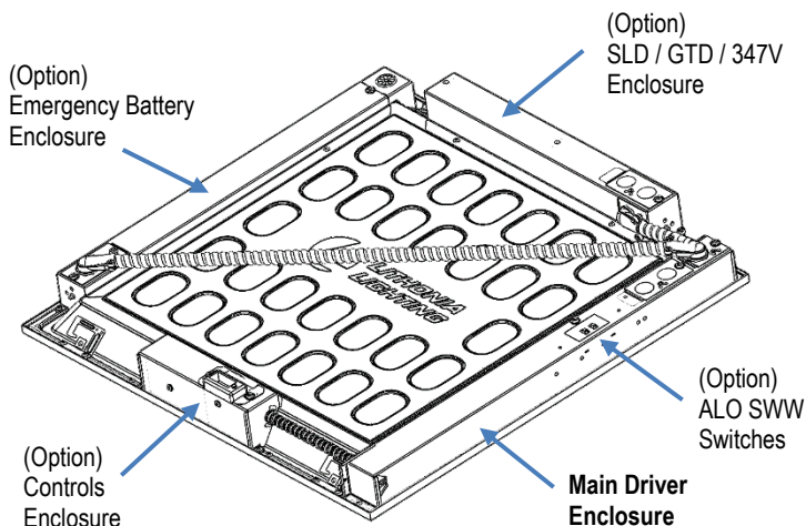
FIG 2: BACK OF FIXTURE
