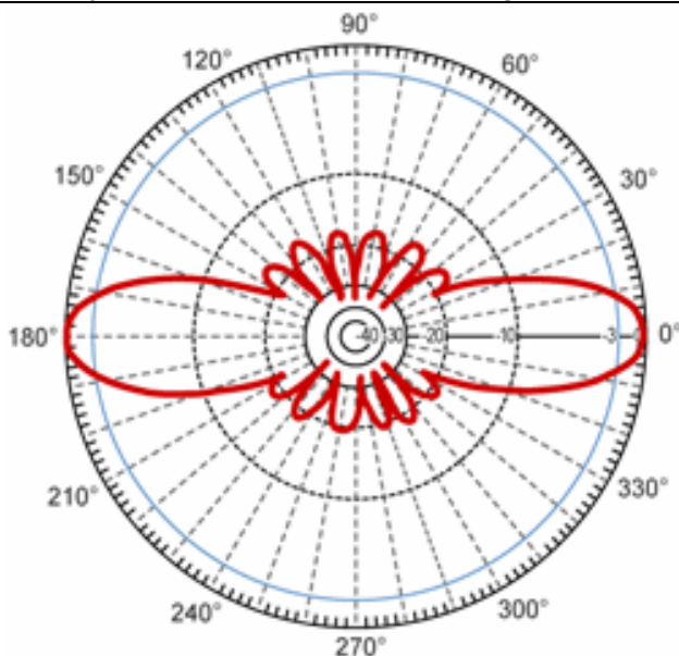
Vertical Pattern
