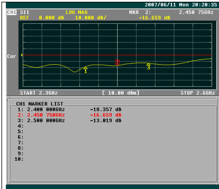
Return loss
