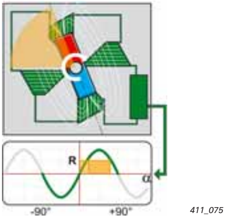
A resistance value produces two possible angles of rotation.
