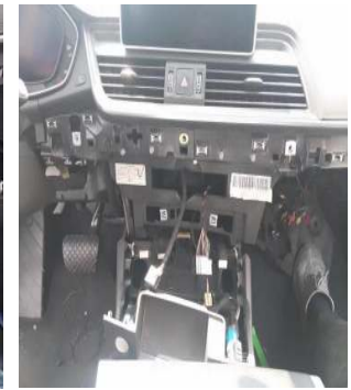
取下空调面板后再取下 后面的螺丝/Remove the air conditioning panel and then remove the screws at the back
