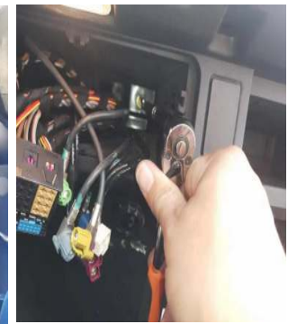
取下主机后，再把主机后面的储物盒固定螺丝取下/After removing the host, remove the screws securing the storage box at the back of the host
