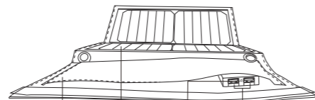
Device Charging Compartment Solar Panel LED Charging Indicator USB Charging Ports
