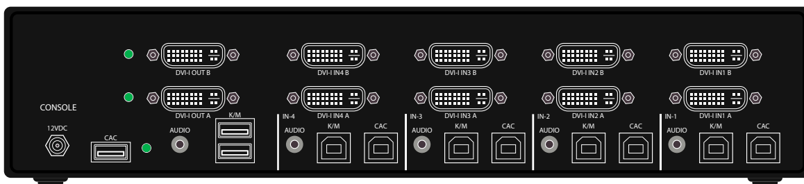
Figure 1-2: KVS4-2004DX Rear panel
