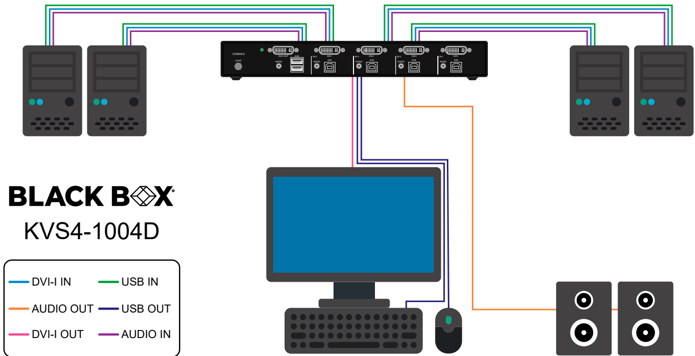
Figure 1-3: KVS4-1004D
