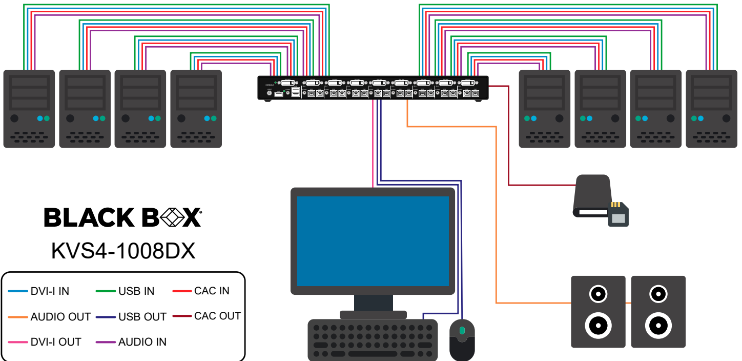
Figure 1-7: KVS4-1008DX
