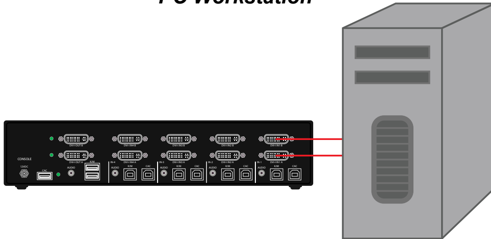
Figure 1-4: KVS4-2004DX
