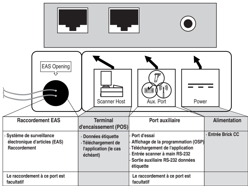
Figure 3. Raccordement
