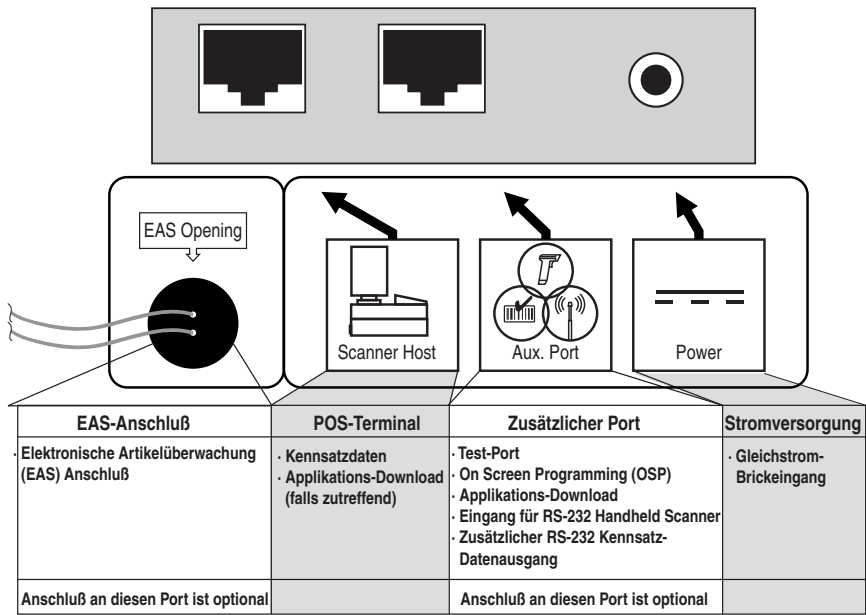
Figure 5. Anschlüsse
