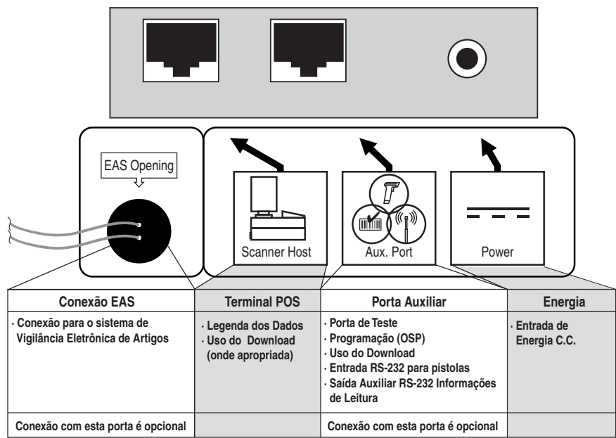
Figure 11. Conexões
