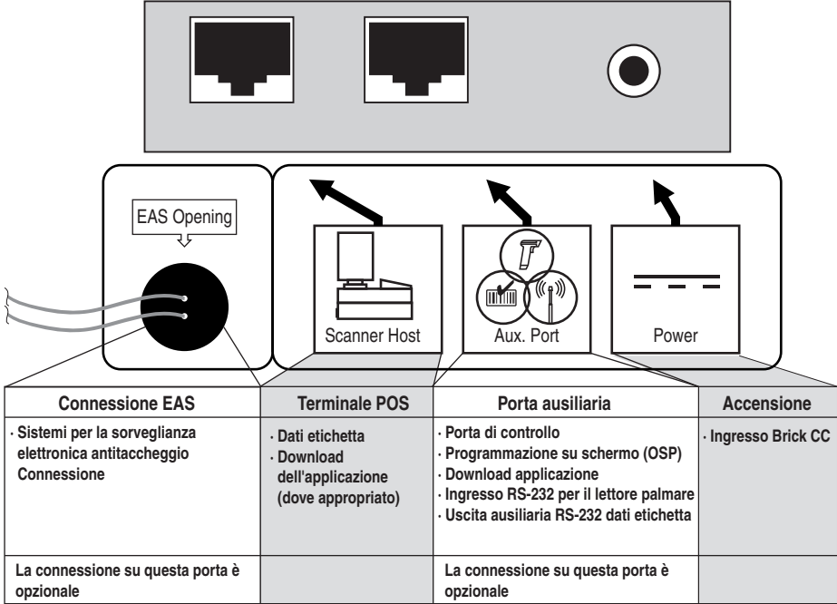
Figure 7. Connessioni
