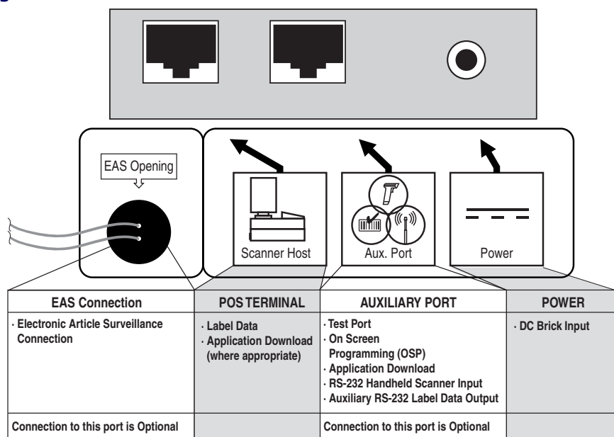
Figure 1. Connections
