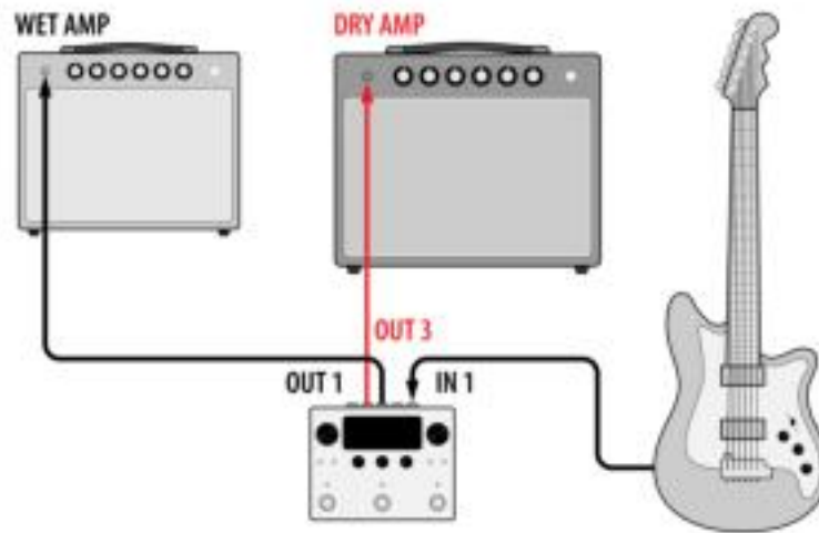
Fig. 3.6 Wet/Dry guitar amp configuration
