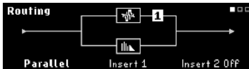
Fig. 3.8 The tap position of the dry amp is post-Preset A in Parallel
