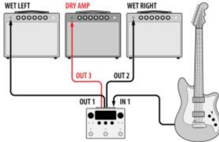
Fig. 3.9 Wet/Dry/Wet guitar amp configuration
