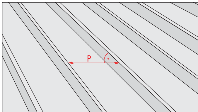
Fig.12. P- Distance between the ceiling joists.
