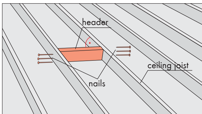
Fig.13. Nail the header at both ends.
