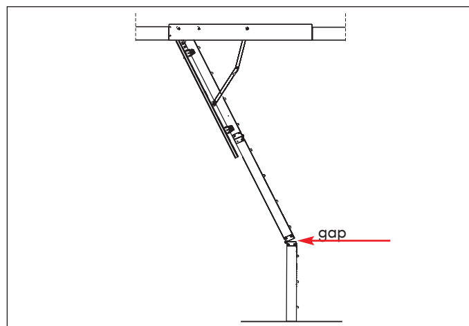
Fig.33. Legs too short.
