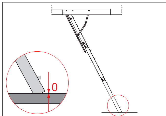
Fig.31. Properly installed attic ladder
