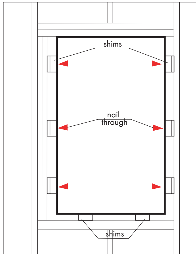
Fig.25. View from the top.
