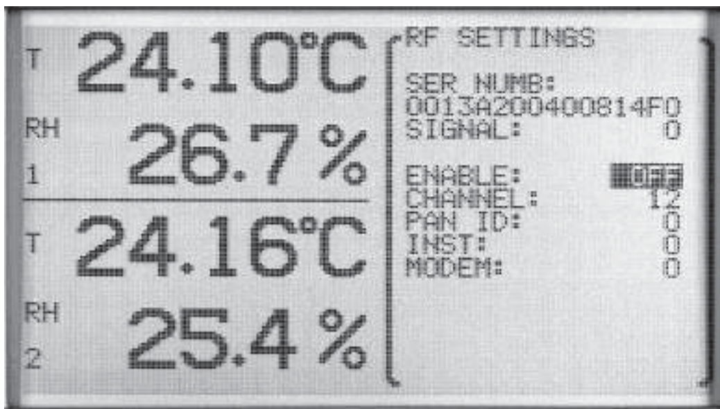
Figure 44 RF Settings
