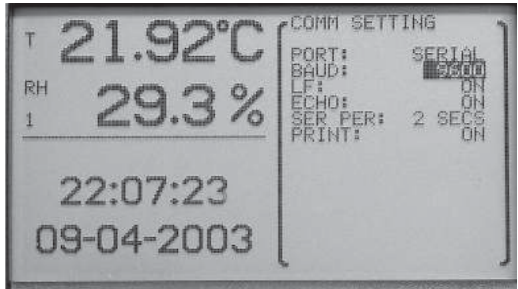
Figure 43 Serial
