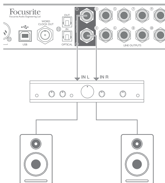
Passive Speakers
