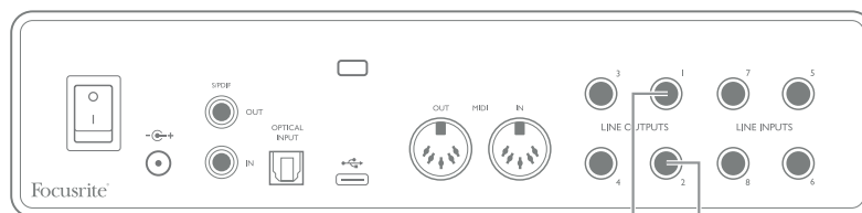
Connecting to Passive speakers
