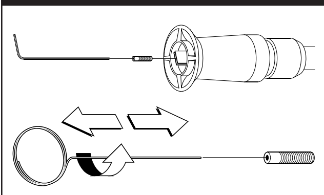
Figure 14 — Removing and cleaning the nozzle.
