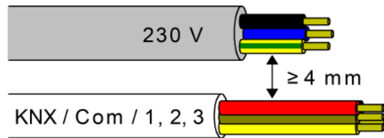
Figure 4: Cable spacing
