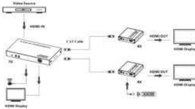
Figure 4: Application Diagram
