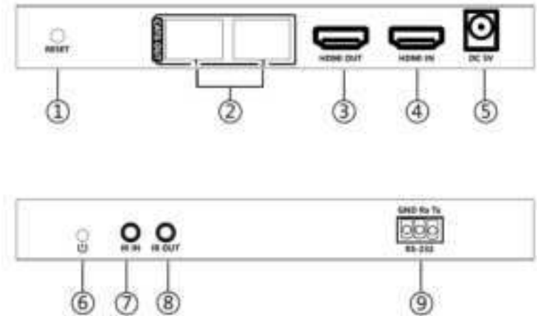
Figure 1: Transmitter Layout
