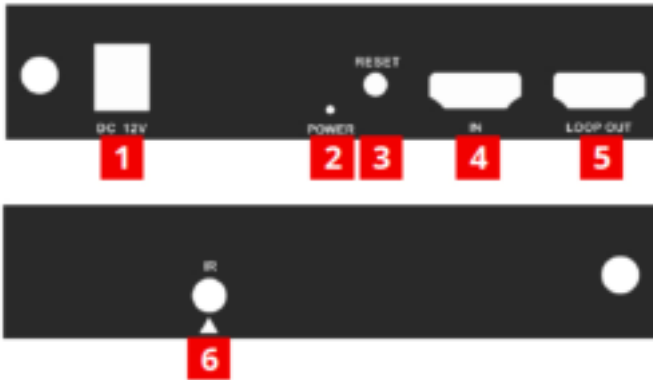
Figure 1: Transmitter (TX)
