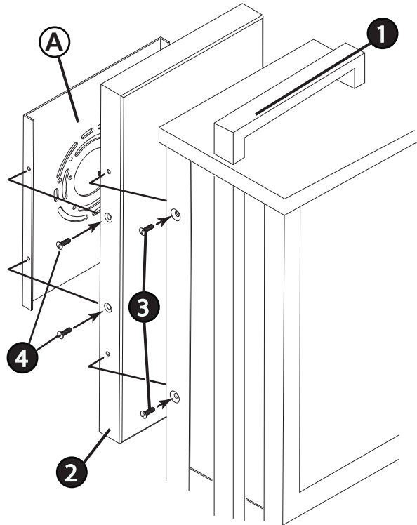
DRAWING 2 - MOUNTING
