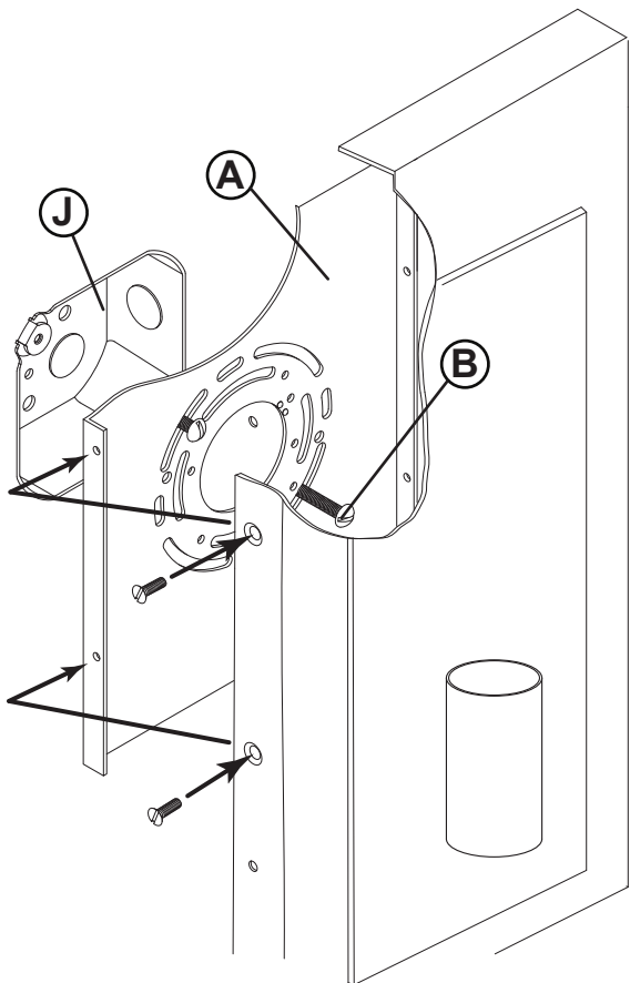
DRAWING 2 - MOUNTING
