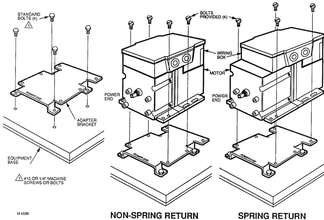
Fig. 1. Damper Application. First mount adapter bracket to equipment, then mount motor to bracket using bolts provided.
