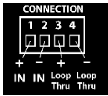
Figure 6 Connector Pins
