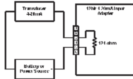
Non-switched Connection
