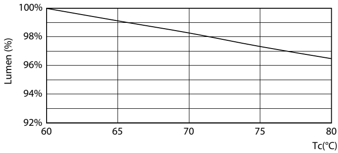
Lumen Maintenance Diagram - MAS LEDtube VLE 1200mm HO 13.5W865 T8
