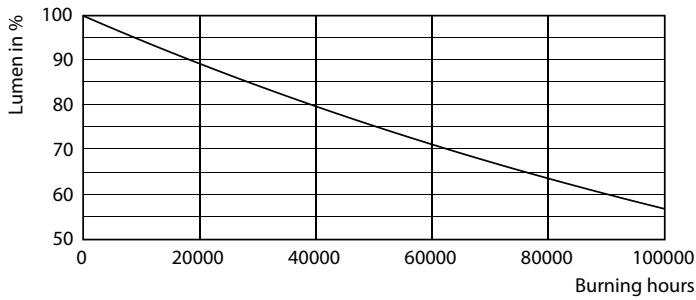
Lumen Maintenance Diagram - MAS LEDtube VLE 1200mm HO 13.5W865 T8
