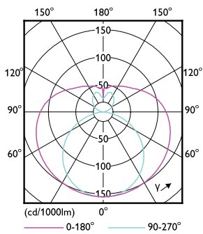
Light Distribution Diagram - MAS LEDtube VLE 1200mm HO 13.5W865 T8
