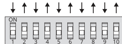
DIP Switches on Receiver 300 (default positions)
