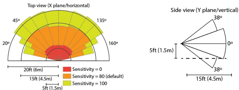
Figure 3: PIR Sensitivity
