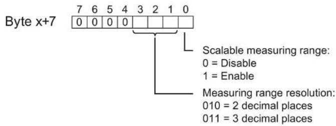
Figure A-5 Structure DS128 AI8 Byte x+7
