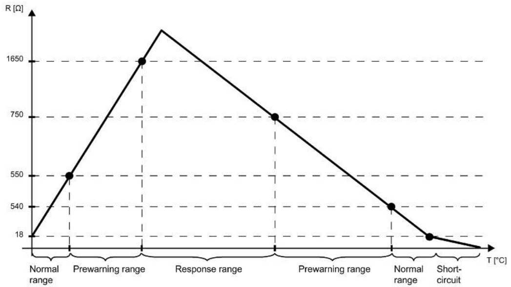
Figure 5-2 Temperature curve with prewarning range
