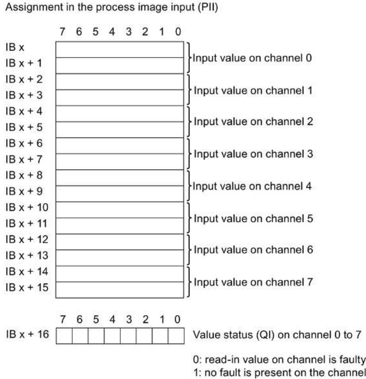
Figure 5-10 Address space of the AI 8xRTD/TC 2-wire HF with value status
