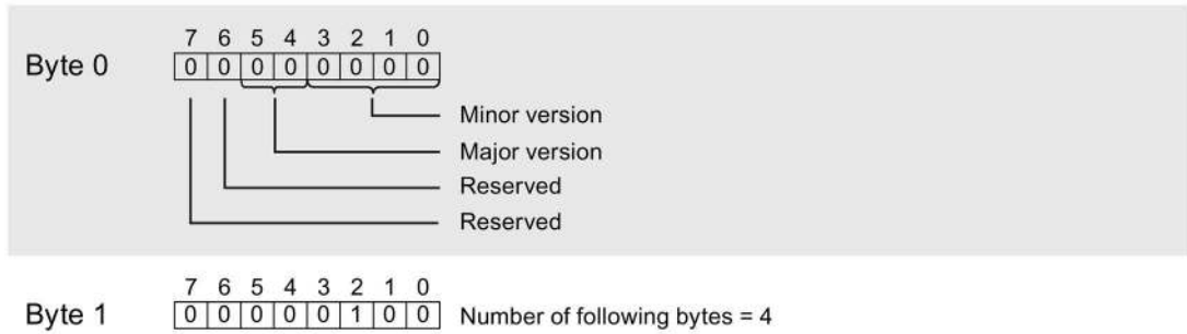
Figure 6-2 Header information
