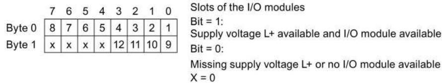
Figure 3-1 Configuration with enabled status detection of the supply voltage L+ (2 bytes)
