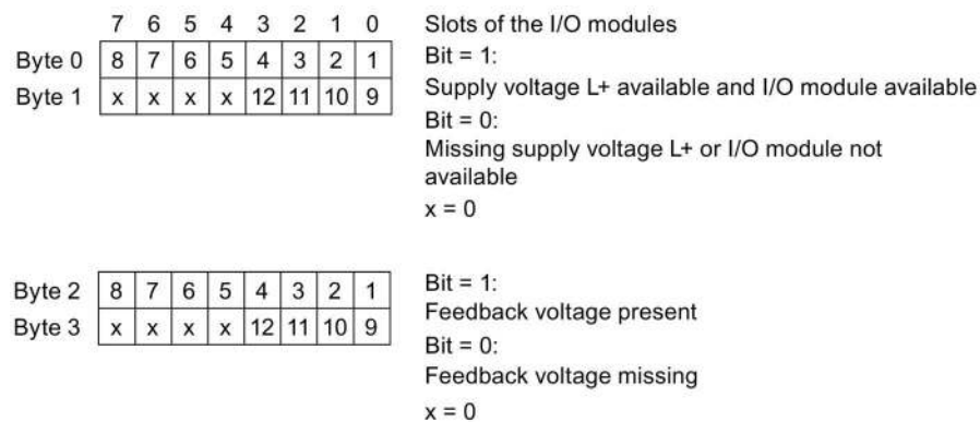
Figure 3-2 Configuration with enabled status detection of the supply voltage L+ and enabled status detection of the feedback voltage (4 bytes of input data)
