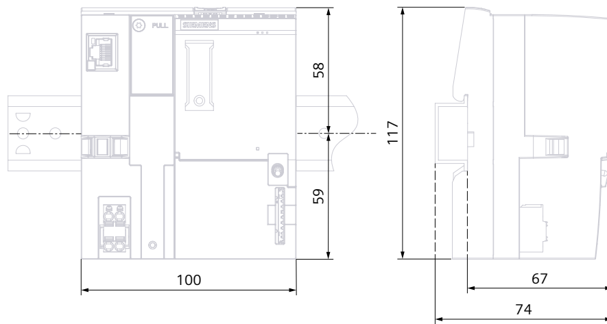
Figure A-1 Dimension drawing CPU 1512SP-1 PN
