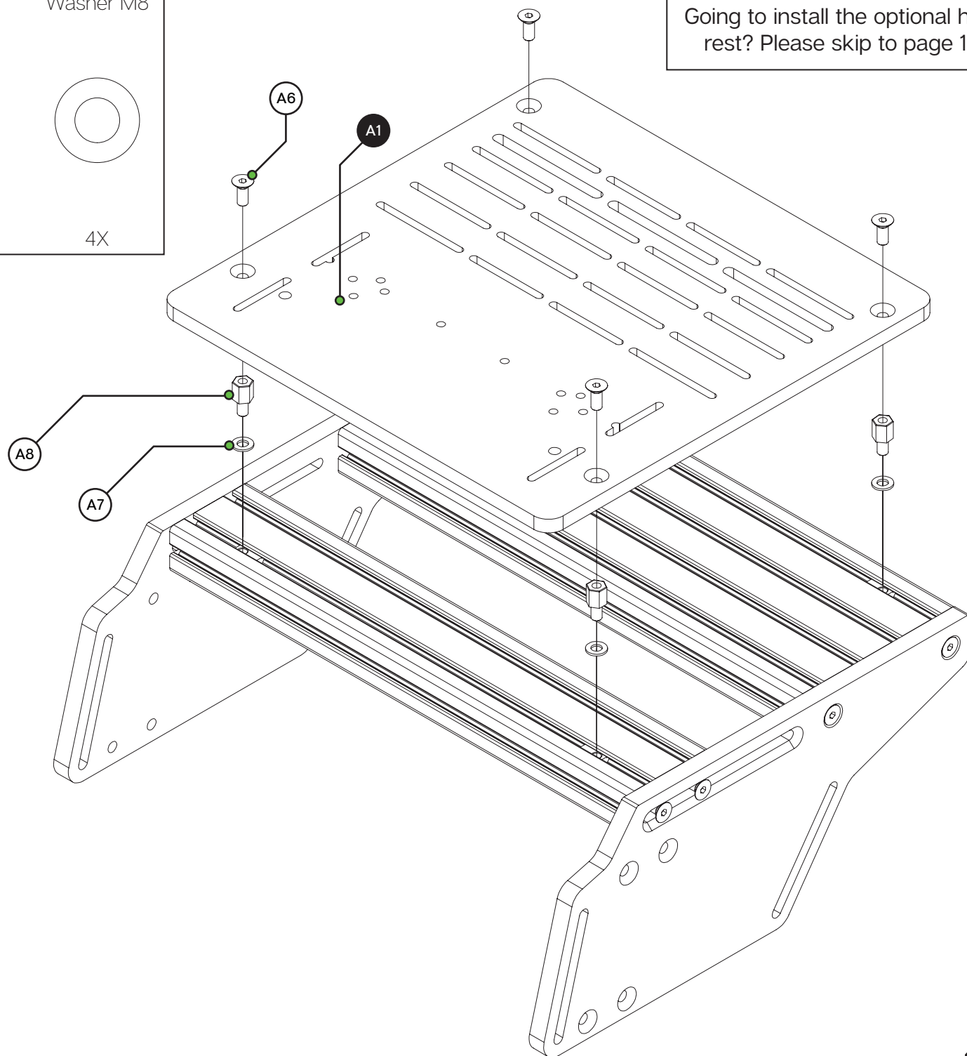
Washer M8
