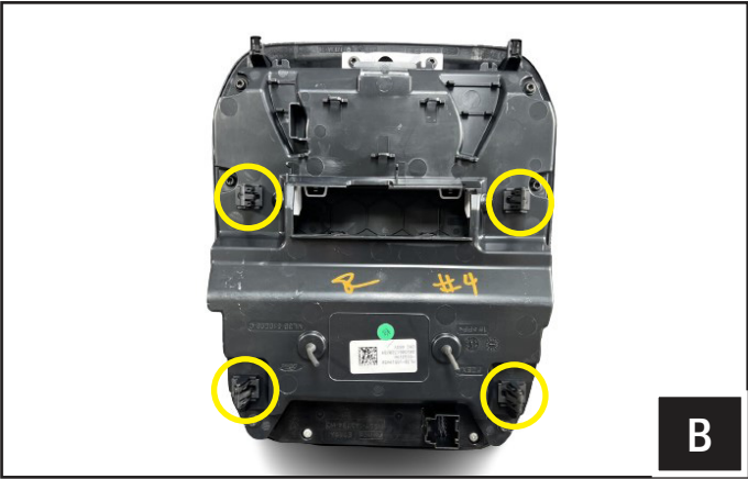
B. Note that there are 4 clips that secure the overhead console to the headliner.
