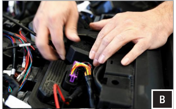
B. Mount the LIT-CC RGB LED Controller Command Center in the dash away from moving parts and secure with zip ties. Cut excess zip ties for a clean install.
