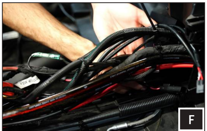
F. Run the rear speaker, subwoofer cable along the passenger side of the center console. Use zip ties to tidy up the install.
