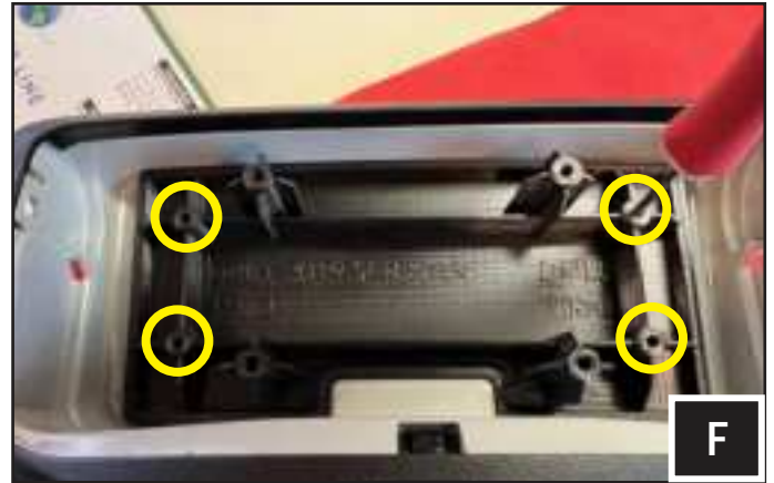
F. Lay the Sprinter mounting bracket in the sunglasses holder cavity and mark screw holes using a pick tool.
