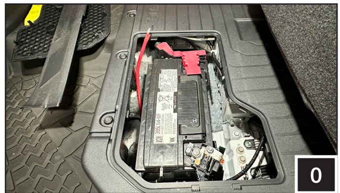
O. Cut the power cable and install the provided fuseholder no more than 18" away from the ring terminal. NOTE that the 15 button controller MUST be plugged in to the module before connecting the power cable to the battery.
