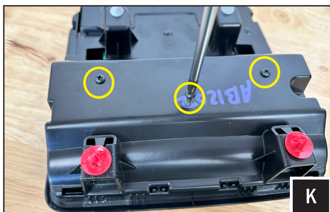
K. Flip the overhead console upside down and use (3) #7-19x3/4" Phillips screws (B-S1656) to secure the bracket.
