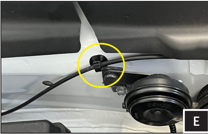
E. Remove the hood release cable from the cable clamp.
