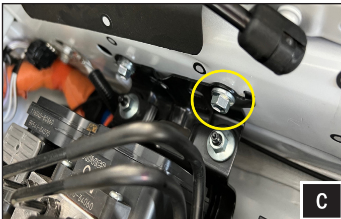
C. Remove the front bolt of the ABS pump bracket using a 12mm wrench.
