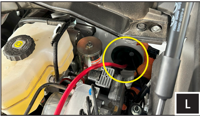
L. Fish the 4 gauge power wire through the firewall grommet towards inside the cabin .
