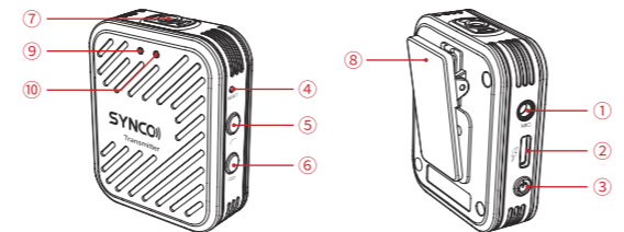
TX Transmitter
