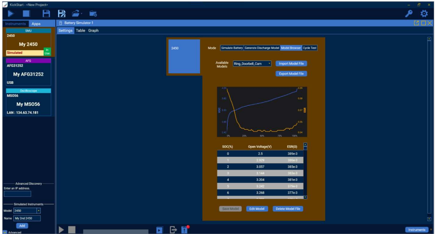
Figure 16: Model Browser
