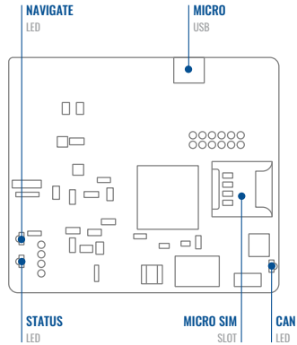
BOTTOM VIEW (WITHOUT COVER)
