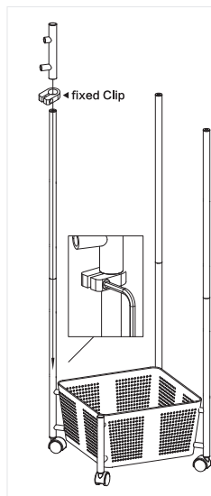
3. Install fixed clip and put the rotary tube in, one rotary tube must have one fixed clip to avoid it run up and down.
