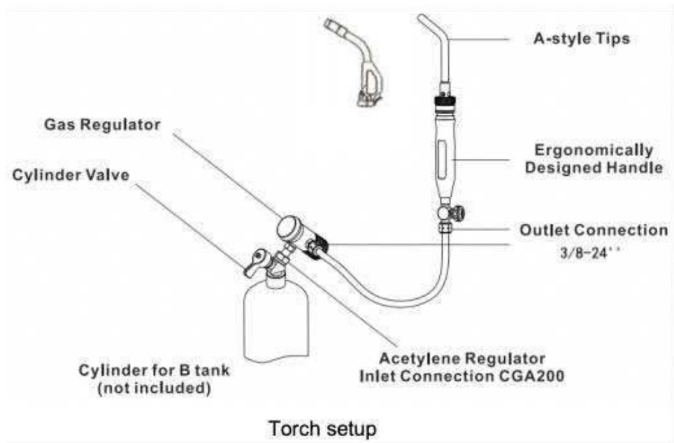
Torch setup
