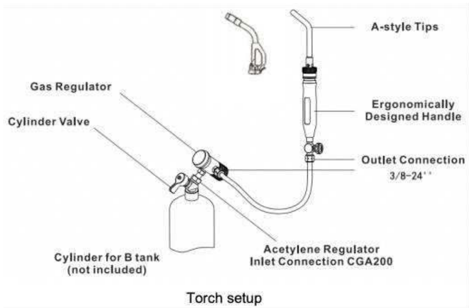
Torche installation
