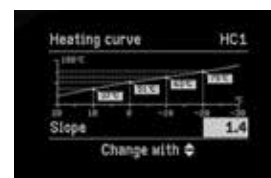
Example: Vitotronic 200 HO1B heating curve
