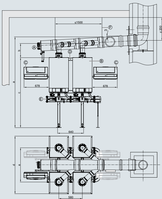
Shown without the thermal insulation supplied
