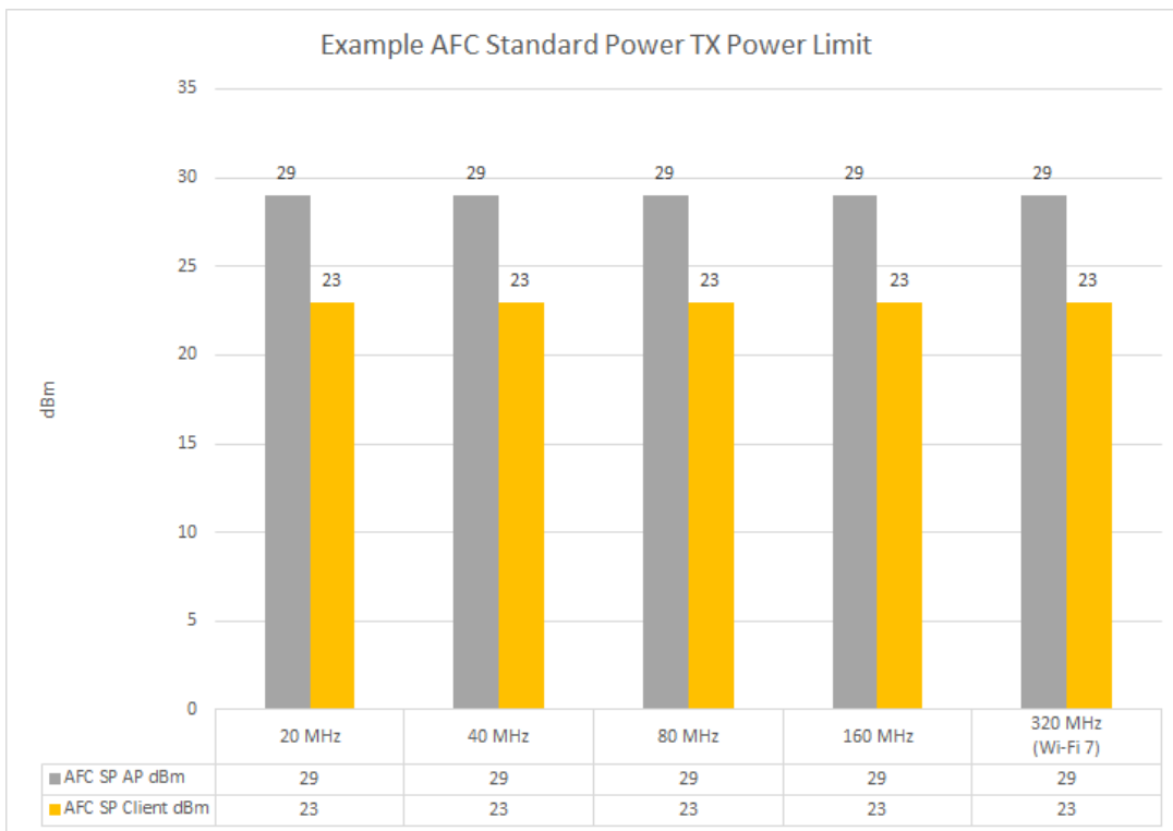
Figure 7 AFC Standard Power TX Power Limit
